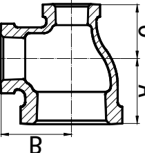
Reducing Tee
