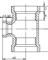
Reducing Tee
