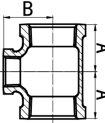
Reducing Tee
