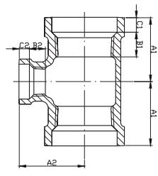
Reducing Tee
