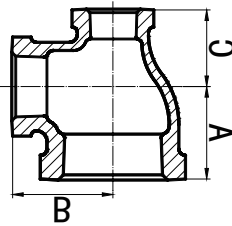
Reducing Tee
